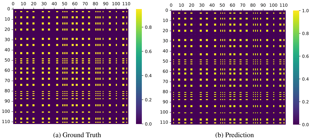
Figure 5: Joint class-specific of concepts importance heatmap ( p(c_{k'} = 1, c_k = 1|\mathbf{y}) ) for ECBM’s ground truth and prediction derived from Proposition 3.3.
