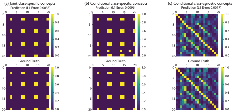
Figure 4: We selected the class “Black and White Warbler” in CUB for illustration. (a) Joint class-specific concept importance p(c_{k'} = 1, c_k = 1|\mathbf{y}) for ECBM’s prediction and ground truth derived from Proposition 3.3. (b) Class-specific conditional probability among concepts p(c_k = 1|c_{k'} = 1, \mathbf{y}) for ECBM’s prediction and ground truth derived from Proposition 3.4. (c) Class-agnostic conditional probability among concepts p(c_k = 1|c_{k'} = 1) for ECBM’s prediction and ground truth derived from Proposition 3.5.
