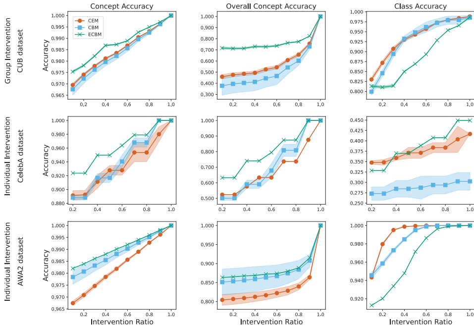
Figure 2: Performance with different ratios of intervened concepts on three datasets (with error bars). The intervention ratio denotes the proportion of provided correct concepts. We use CEM with RandInt. CelebA and AWA2 do not have grouped concepts; thus we adopt individual intervention.
