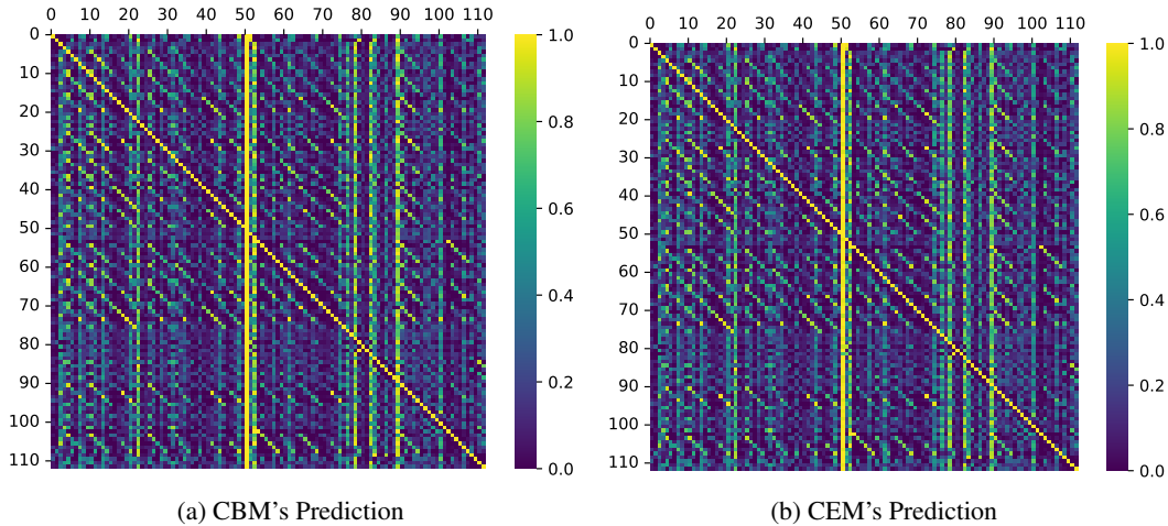
Figure 10: Class-agnostic conditional probability among concepts heatmap ( p(c_k = 1 | c_{k'} = 1) ) for CBM's and CEM's predictions.
