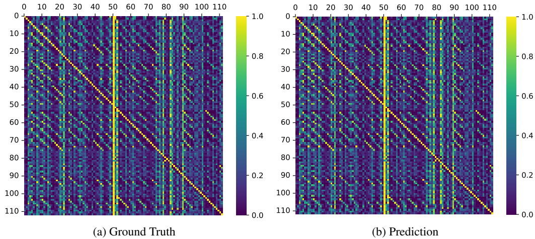
Figure 7: Class-agnostic conditional probability among concepts heatmap ( p(c_k = 1 | c_{k'} = 1) ) for ECBM’s ground truth and prediction derived from Proposition 3.5.
