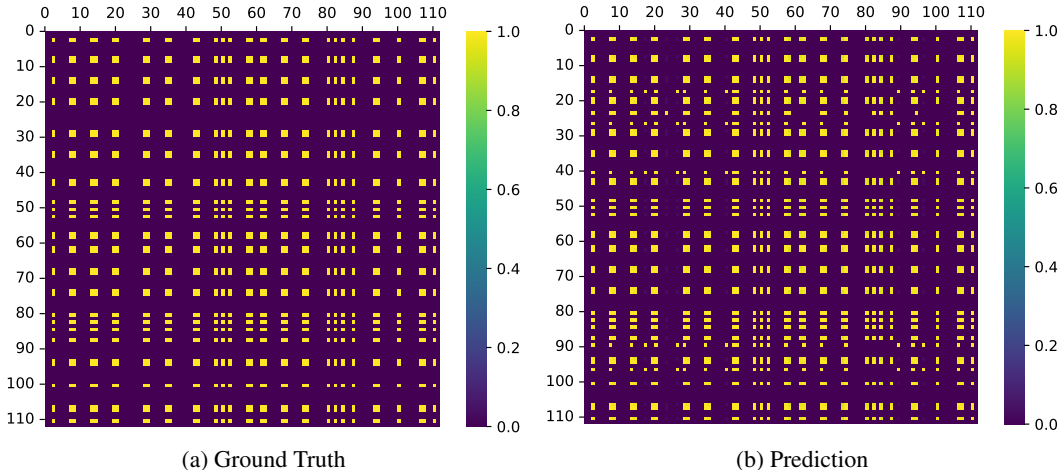
Figure 6: Class-specific conditional probability among concepts heatmap p(c_k = 1|c_{k'} = 1, \mathbf{y}) for ECBM’s ground truth and prediction derived from Proposition 3.4.
