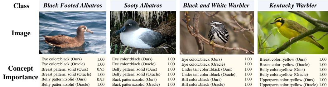
Figure 3: Marginal concept importance ( p(c_k = 1|\mathbf{y}) ) for top 3 concepts of 4 different classes computed using Proposition 3.2. ECBM’s estimation (Ours) is very close to the ground truth (Oracle).
