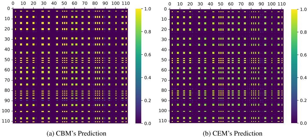
Figure 8: Joint class-specific of concepts importance heatmap ( p(c_{k'} = 1, c_k = 1 | \mathbf{y}) ) for CBM's and CEM's predictions.
