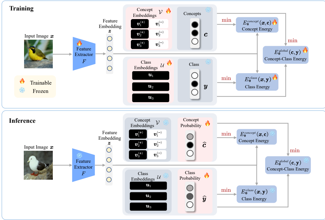
Figure 1: Overview of our ECBM. Top: During training, ECBM learns positive concept embeddings v_k^{(+)} (in black), negative concept embeddings v_k^{(-)} (in white), the class embeddings u_m (in black), and the three energy networks by minimizing the three energy functions, E_\theta^{class}(\mathbf{x}, \mathbf{y}) , E_\theta^{concept}(\mathbf{x}, \mathbf{c}) , and E_\theta^{global}(\mathbf{c}, \mathbf{y}) using Eqn. 1. The concept \mathbf{c} and class label \mathbf{y} are treated as constants. Bottom: During inference, we (1) freeze all concept and class embeddings as well as all networks, and (2) update the predicted concept probabilities \hat{\mathbf{c}} and class probabilities \hat{\mathbf{y}} by minimizing the three energy functions using Eqn. 1.
