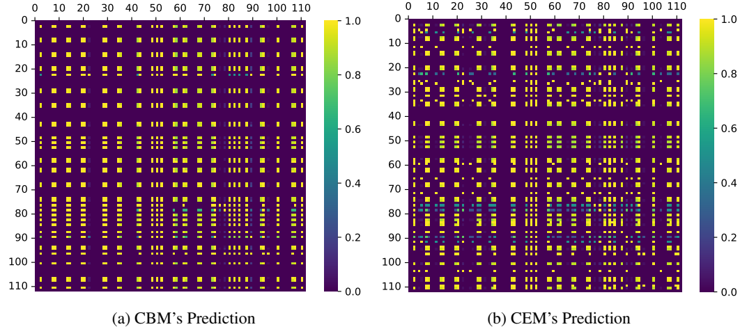
Figure 9: Class-specific conditional probability among concepts heatmap p(c_k = 1 | c_{k'} = 1, \mathbf{y}) for CBM's and CEM's predictions.
