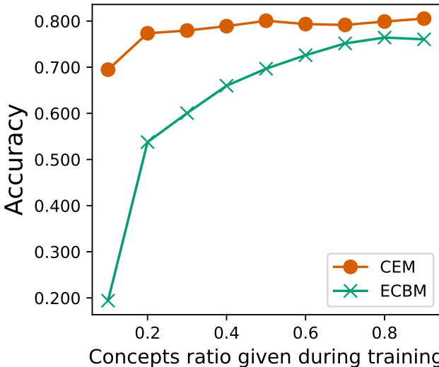
Figure 11: The predictive performance of CEM and hard ECBM on the CUB dataset. The horizontal axis denotes the ratio of concept groups given during the training process, and the vertical axis denotes the “Class Accuracy”.
