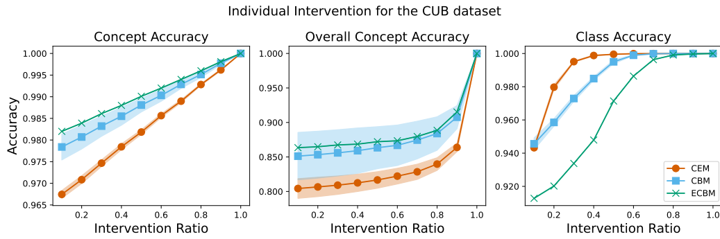
Figure 12: Individual intervention on the CUB dataset (with error bars). The horizontal axis denotes the ratio of the concept group’s ground truth given during the inference process.
