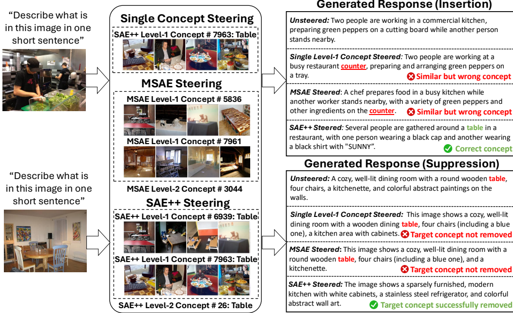
Figure 3: Concept steering on Qwen3-VL-4B-Instruct. We compare unsteered generation, matched Matryoshka SAE steering, the best individual SAE++ Level-1 neuron, and full SAE++ Level-2 clustered steering. In both insertion and suppression, SAE++’s steering most effectively controls the generated response in terms of the “Table” concept.
