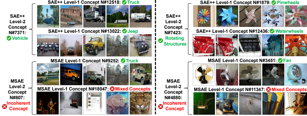
Figure 2: Qualitative examples of multi-level (Level-1 and Level-2) concepts discovered by SAE++ and Matryoshka SAEs (MSAEs). Left: SAE++ groups visually coherent Level-1 concepts, Truck and Jeep , into the same Level-2 concept, Vehicle . In contrast, the matched MSAE concepts are less semantically consistent and often mix weaker or unrelated visual patterns. Right: SAE++ groups visually coherent Level-1 concepts, Pinwheels and Waterwheels , into the same Level-2 concept, Rotating Structures , while the two Level-1 concepts under the same MSAE Level-2 concept are less semantically consistent. Additional qualitative results are provided in Appendix G.
