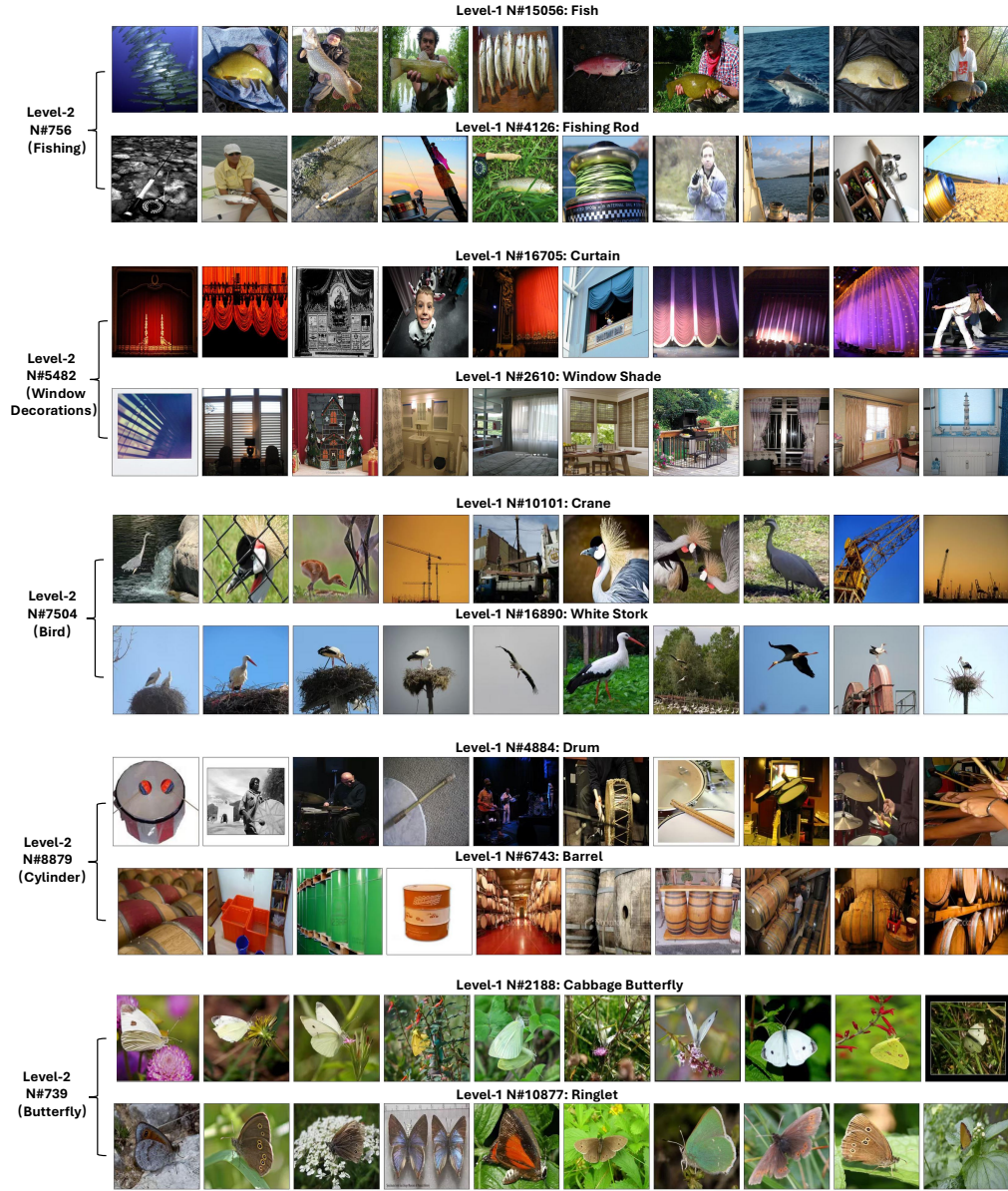
Figure 5: More qualitative results on our SAE++’s learned Level-1 and Level-2 concepts from MLLMs.
